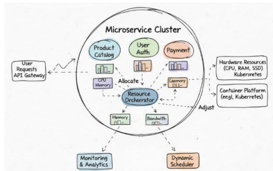
Fig. 6. Microservice Environment for Fine-Grained Resource Allocation
