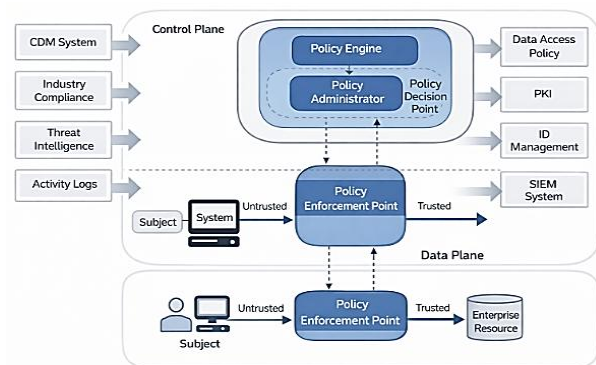
Fig. 1. Logical Components of Zero Trust Model
